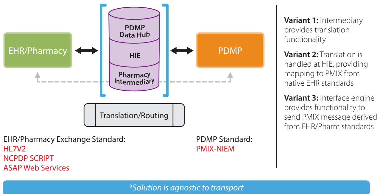
FIGURE 2: EHR, PHARMACY, AND PDMP INTEGRATION
